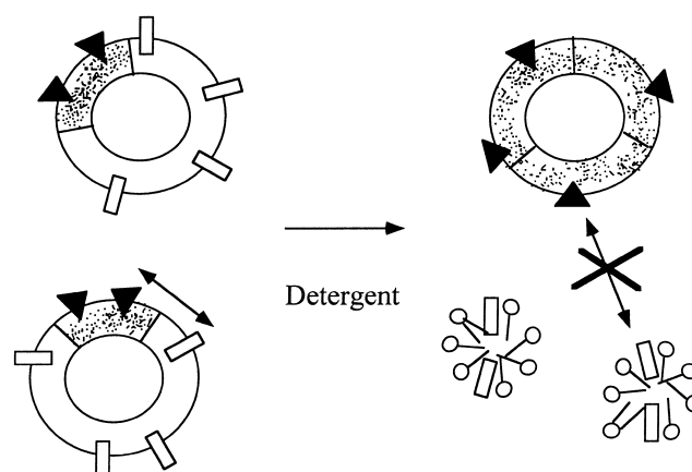
Fig. 5. Schematic illustration of 'trapping' subsequent to the addition of detergent. Shaded regions are bilayer domains in the Lo state. Unshaded regions are in the L \alpha state. Triangles and rectangles represent components that preferentially associate with Lo and L \alpha domains, respectively. Prior to solubilization, components can exchange between coexisting domains by lateral diffusion. After solubilization, exchange cannot occur because it would involve passage of hydrophobic molecules through the aqueous solution.
